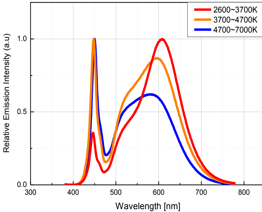
Fig 1. Color Spectrum, T_j = 25^\circ\text{C}
