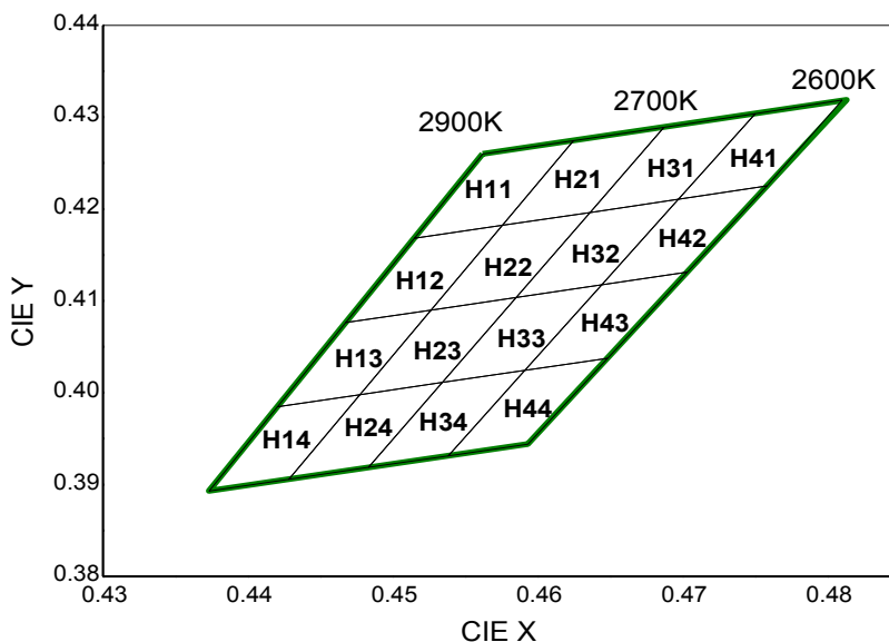
CIE Chromaticity Diagram (Warm white), T_j=25^{\circ}\text{C} , I_F=65\text{mA}
